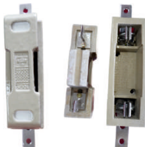
100AMP HANDLE WITH LUGS MSEB TYPE
